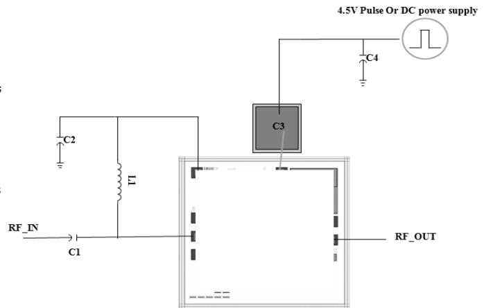
Assembly Diagram
