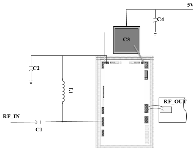
Assembly Diagram
