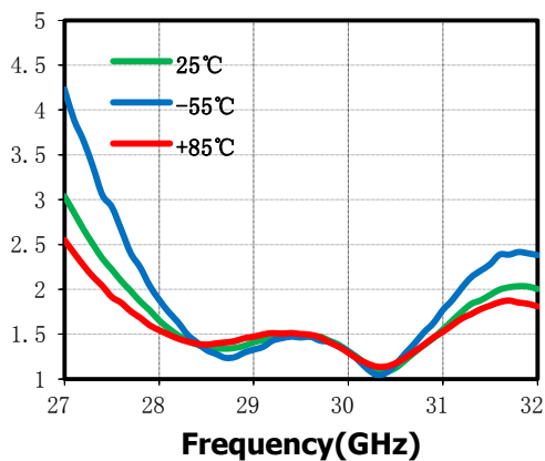
VSWRi(:1) vs.Temperature
