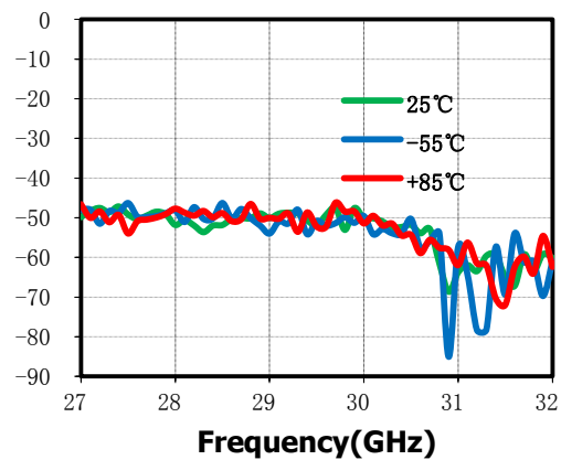
Reverse Isolation(dB)vs.Temperature
