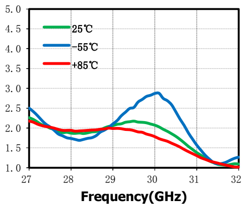
VSWRo(:1) vs.Temperature
