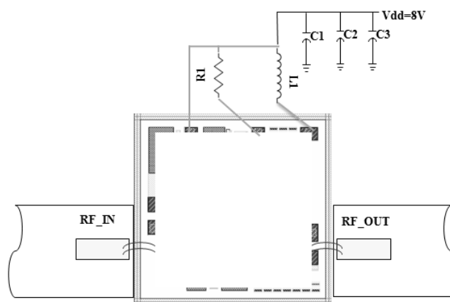
Assembly Diagram
