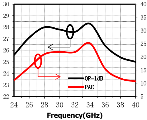
OP 1 dB(dBm), PAE(%) vs.Freq @ V_D=6\text{V}
