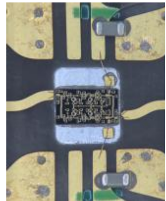
Chip Test Fixture
