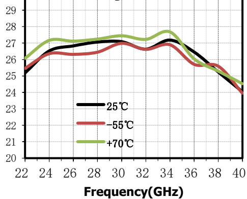
OP 1 dB(dBm) vs.Temperature @ V_D=5\text{V}
