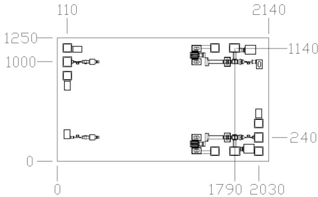
Die Outline (All dimensions in \mu\text{m} )
