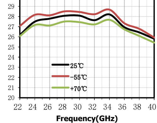
OP 1 dB(dBm) vs.Temperature @ V_D=6\text{V}
