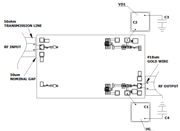
Assembly Diagram
