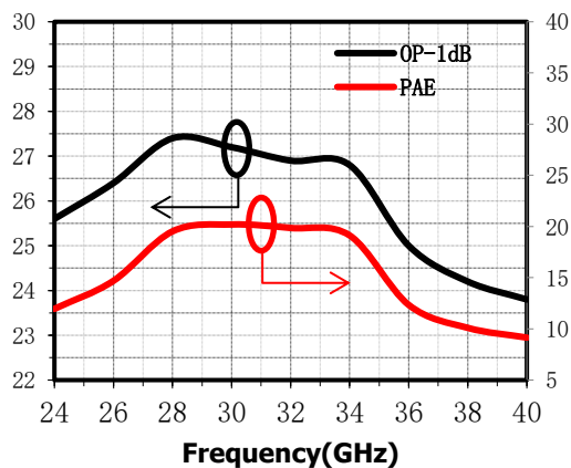
OP 1 dB(dBm), PAE(%) vs.Freq @ V_D=5\text{V}
