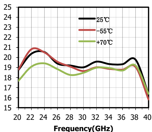
OP 1 dB(dBm) vs.Temperature @ V_D = 5V
