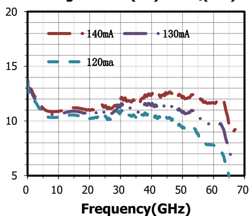
Small Signal Gain(dB) vs.IDQ(mA)
