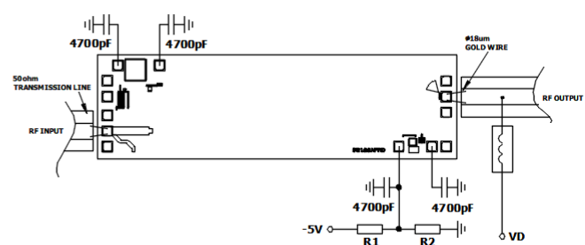
Assembly Diagram
